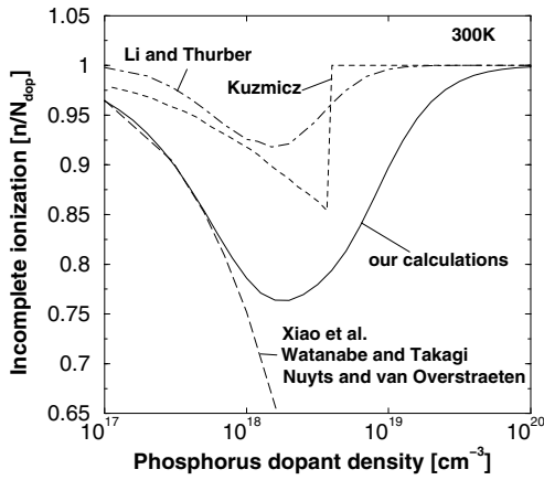
Fig. 3. The fraction of non-ionized phosphorus atoms from various published models compared to the full model of the present paper.
